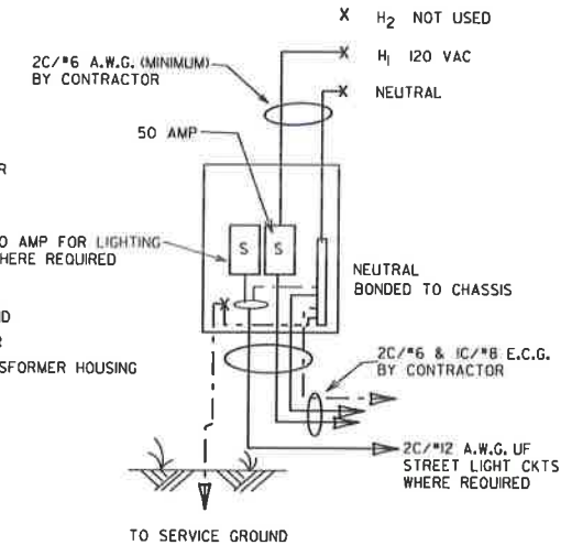
WITHOUT POWER ISOLATION ASSEMBLY 2 CIRCUIT MAIN BREAKER
