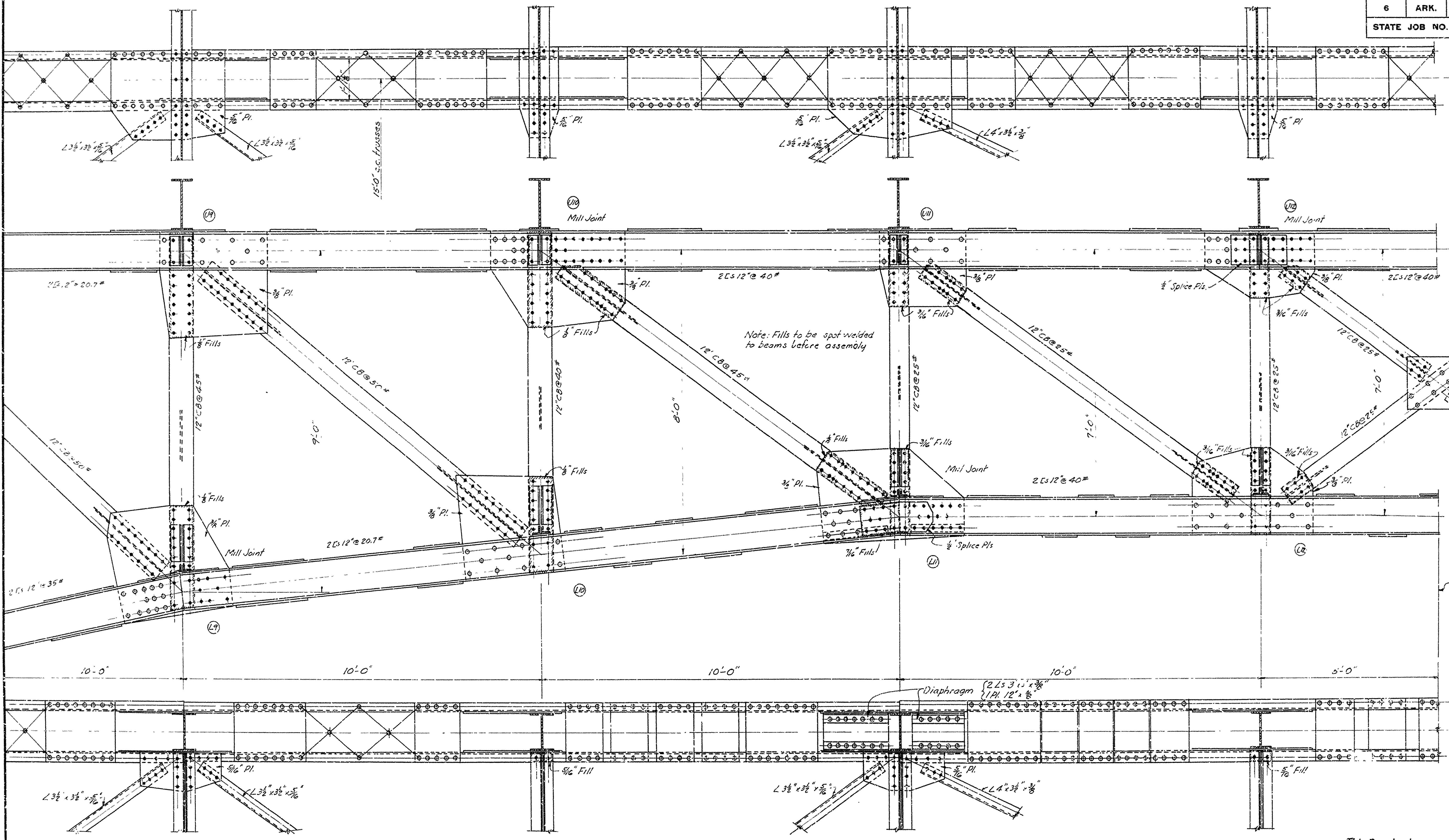
This Drawing to accompany Drawings 2460, 2460-A, and 2460-C DETAILS OF STANDARD 70'-110'-70' CONTINUOUS TRUSS SPANS 24' CLEAR ROADWAY
