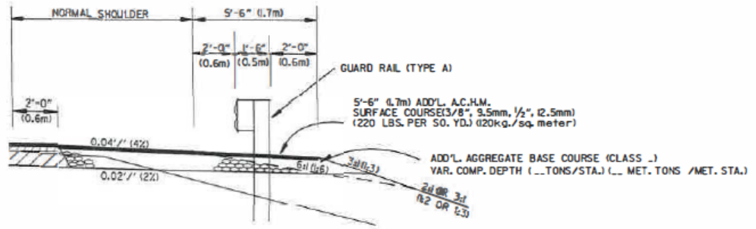
WIDENING FOR GUARD RAIL
