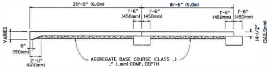
SECTION OF APPROACH SLAB
