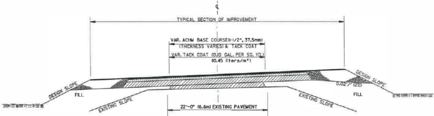
METHOD OF RAISING GRADE
