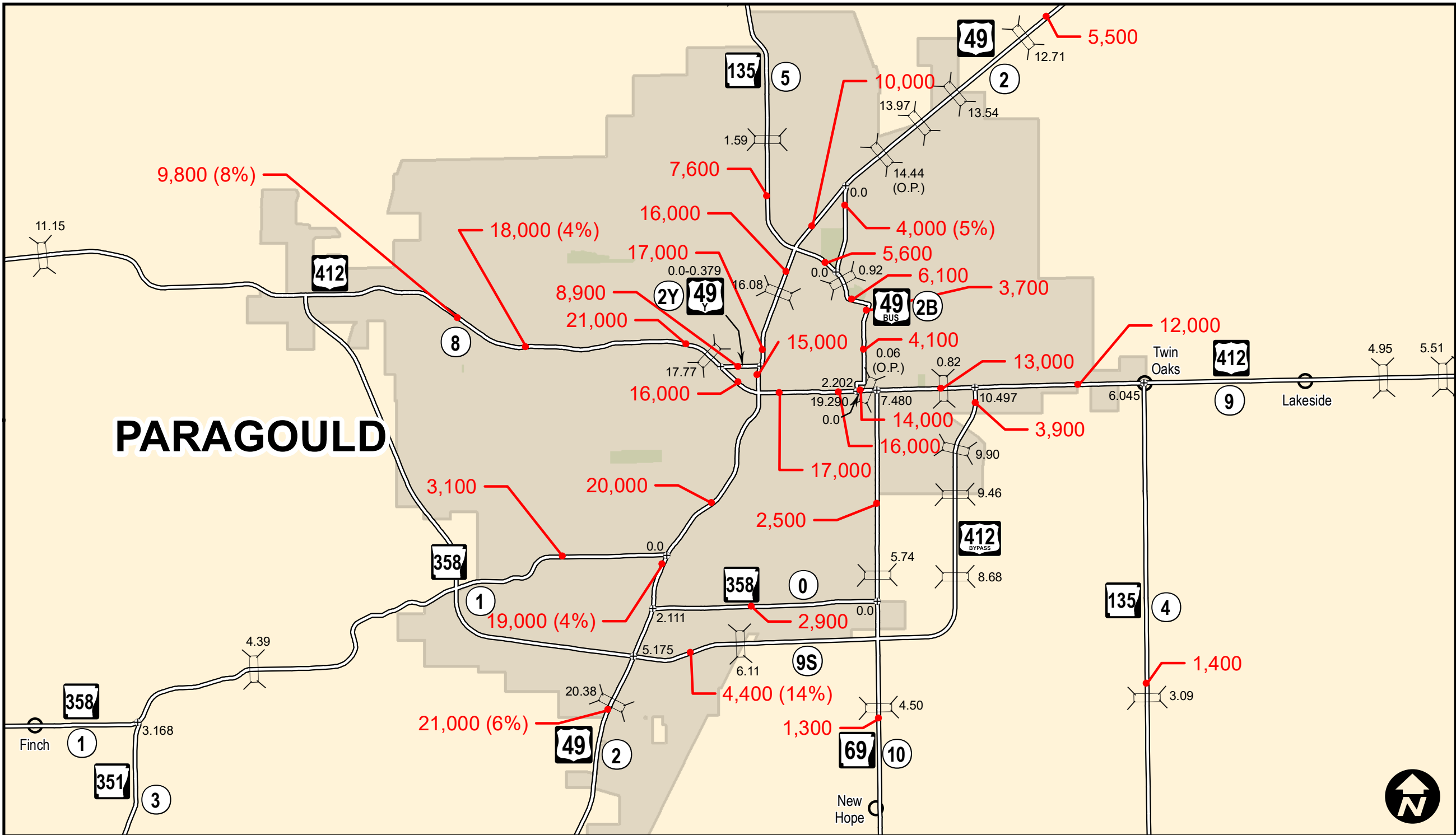
2020 ANNUAL AVERAGE (TRUCK %) DAILY TRAFFIC ESTIMATES
