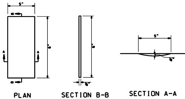
DETAILS OF RUMBLE STRIPE
