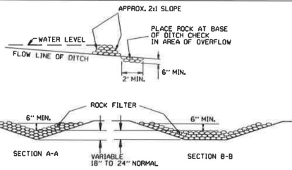
ROCK DITCH CHECK (E-6)
