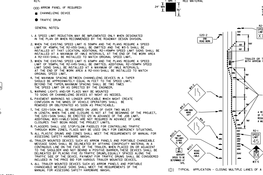
(D) TYPICAL APPLICATION - CLOSING MULTIPLE LANES OF A MULTILANE HIGHWAY.
