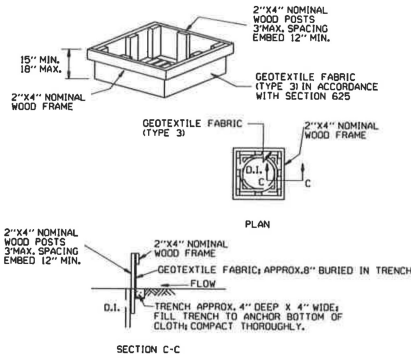
DROP INLET SILTS FENCE (E-7)
