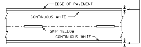
PAVEMENT EDGE LINE MARKING
